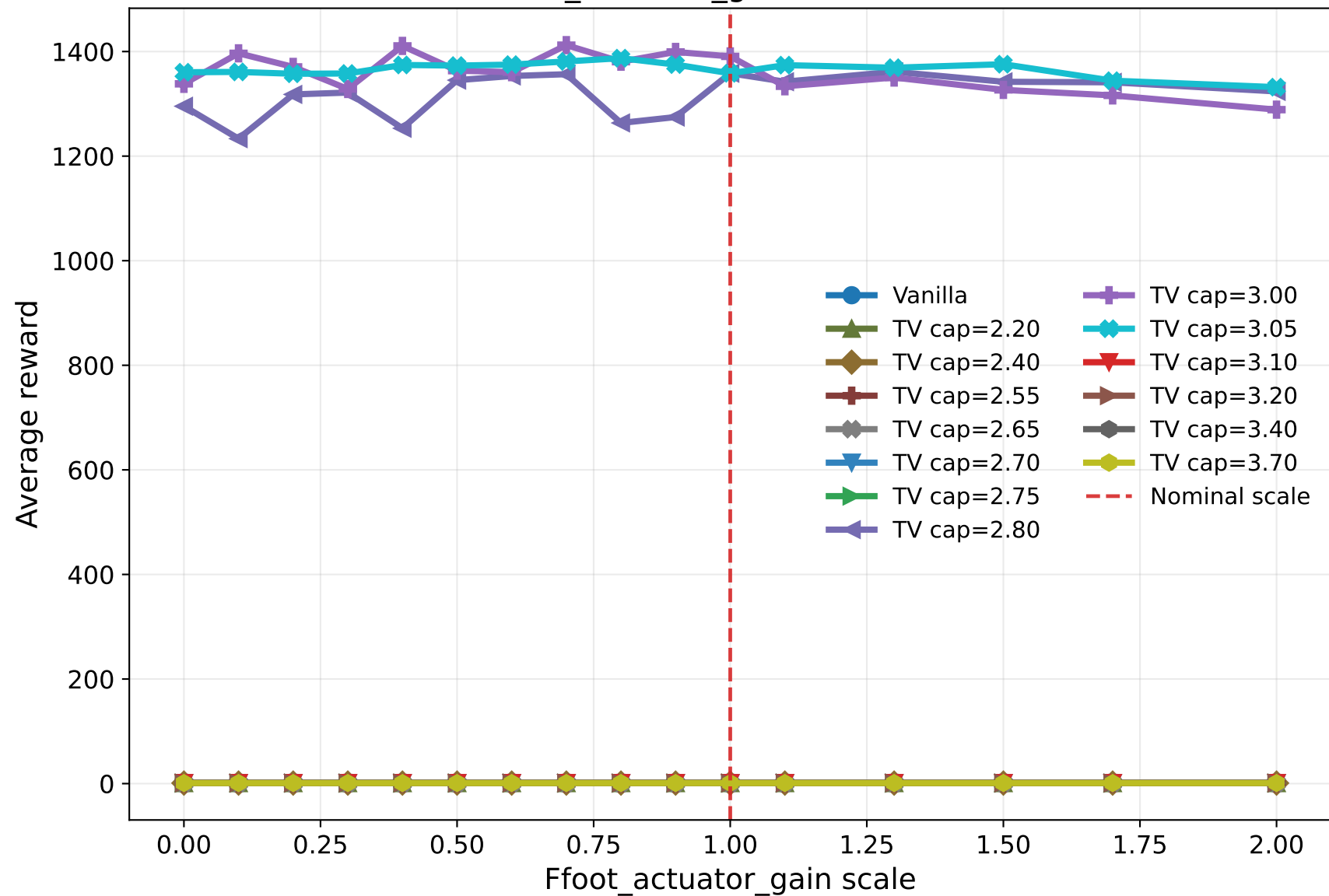
Ffoot_actuator_gain robustness
